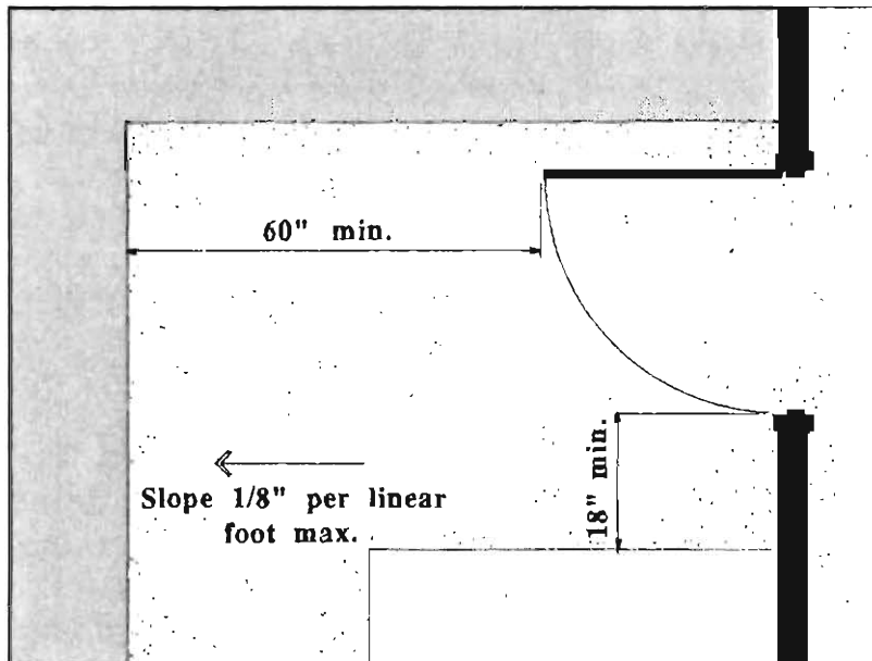
Entrance Landing
