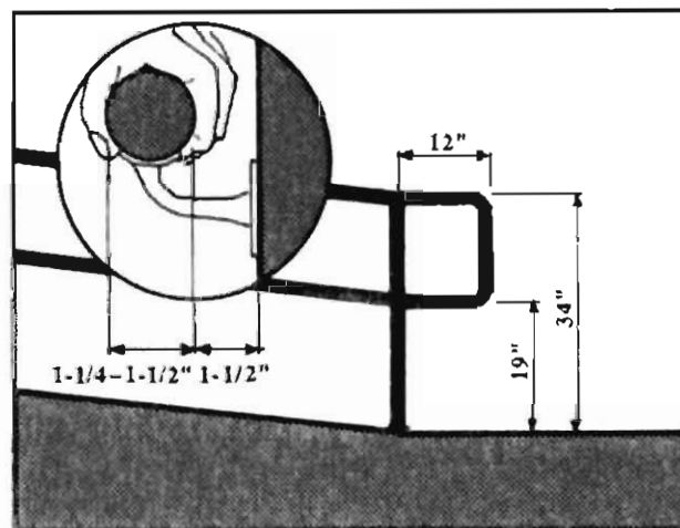
Ramp Handrail With Extensions
