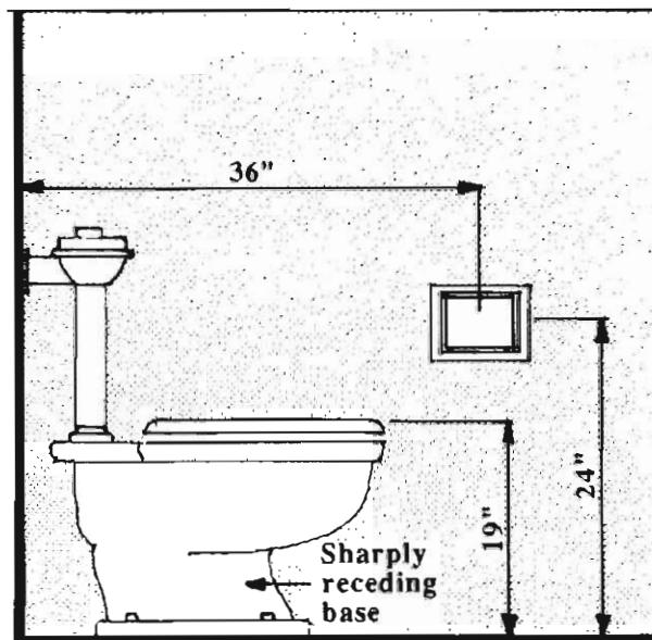
Floor-Mounted Toilet With Receding Base
