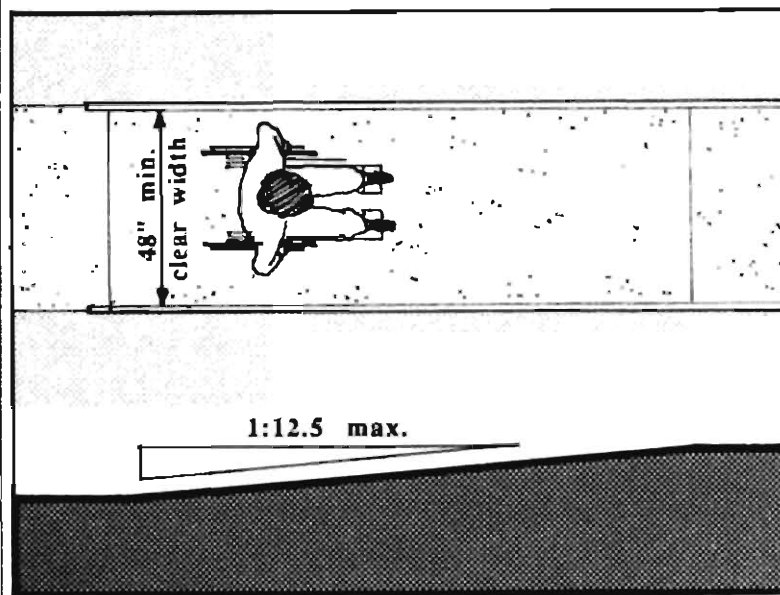
Minimize Slope of Ramps
