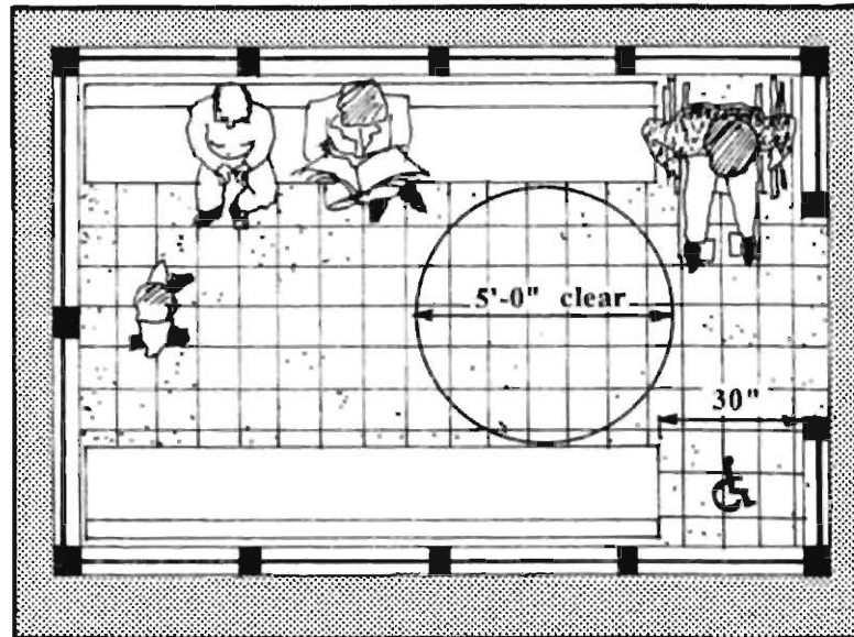
Enclosed Shelter
