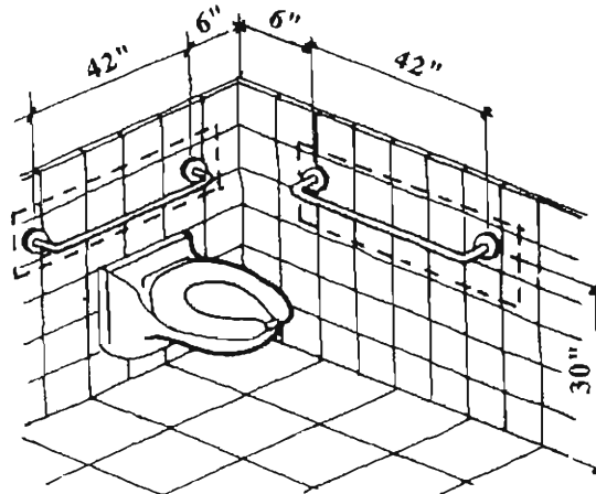
Grab Bar Locations
