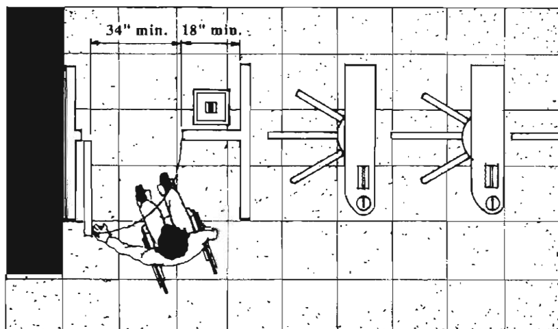
Accessible Gate With 34 Inch Clear Opening and 18 Inch Clearance
