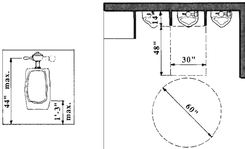
Accessible Urinals
