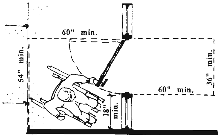
Maneuvering Space at the Door
