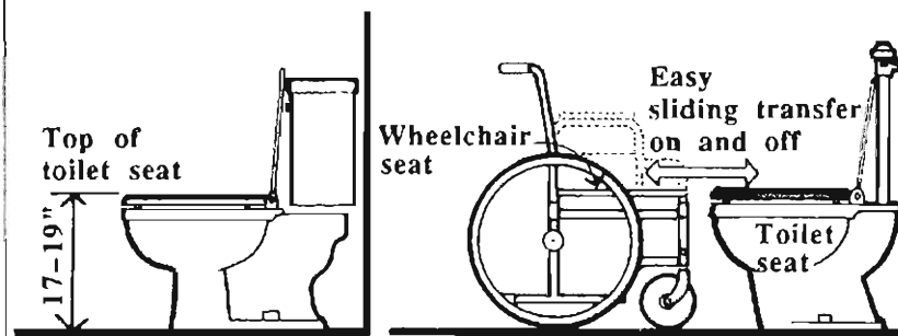
Toilet Seat Height
