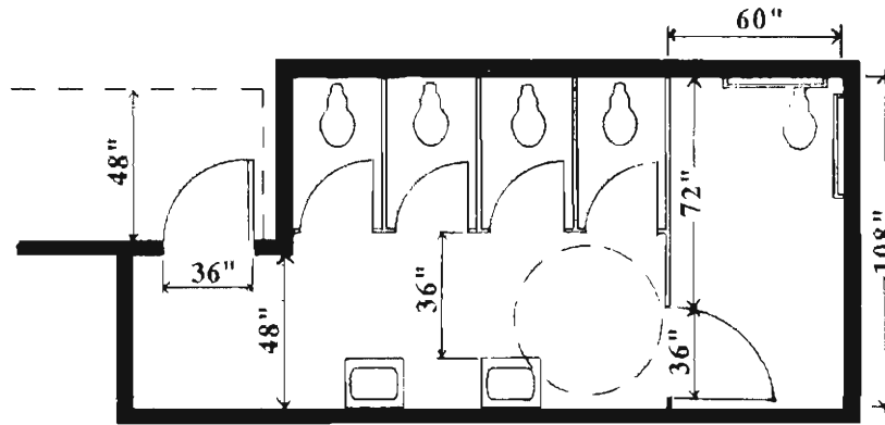
Accessible Toilet Room Layout
