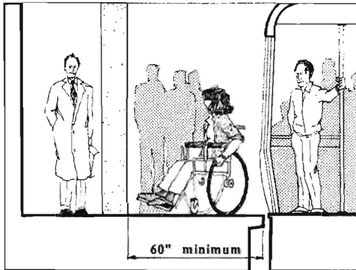
60 Inches Between Platform Edge and Structural Column
