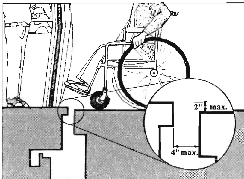
Minimize Gap at Platform/Car Interface
