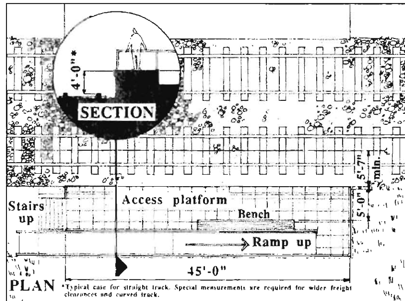
Access Platform Dimensions
