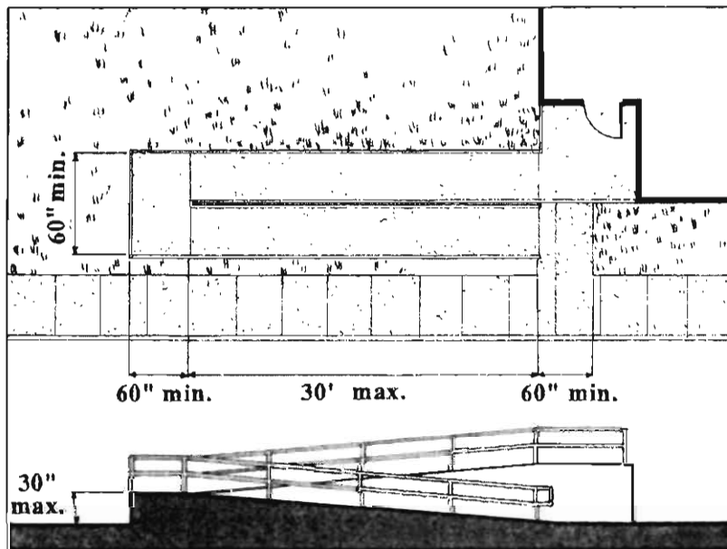
Ramp Landings
