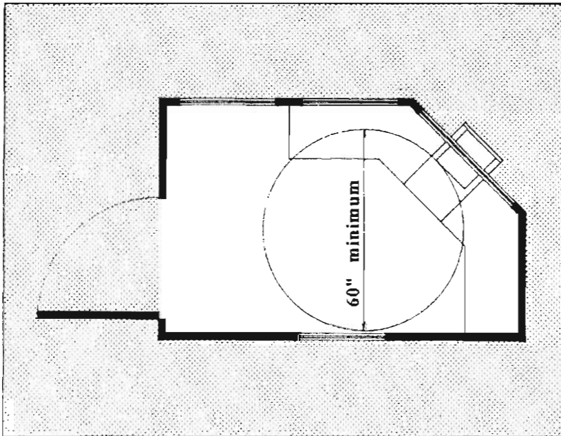
Fare Collection Booth Interior
