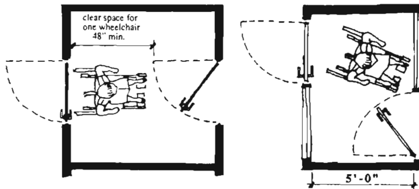
Vestibule Solutions
