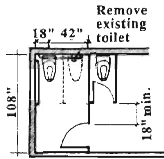
Combining Two Stalls
