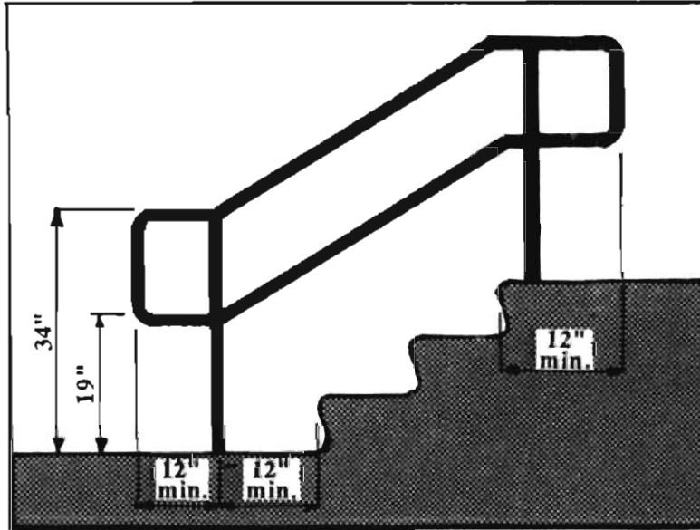
34 Inch and 19 Inch Handrail With Extensions
