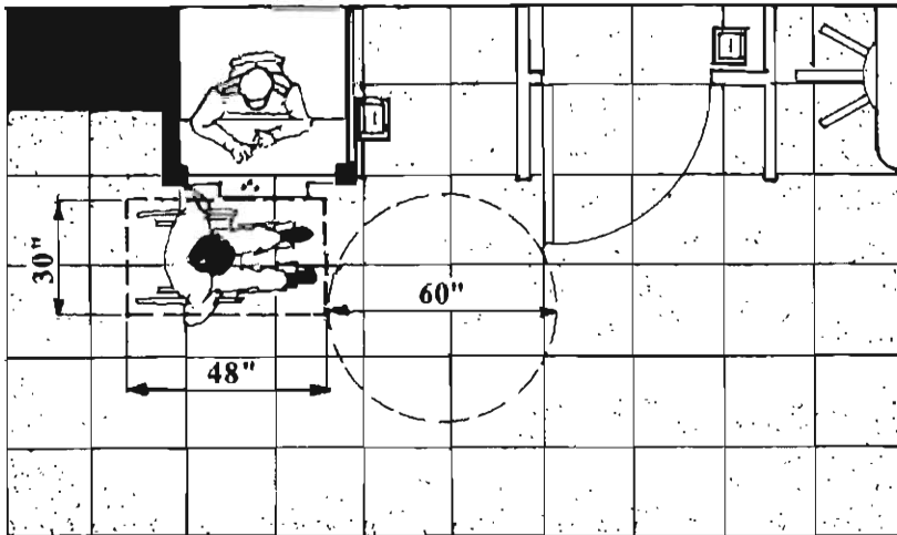
60 x 60 Inch Turning Space Is Necessary
