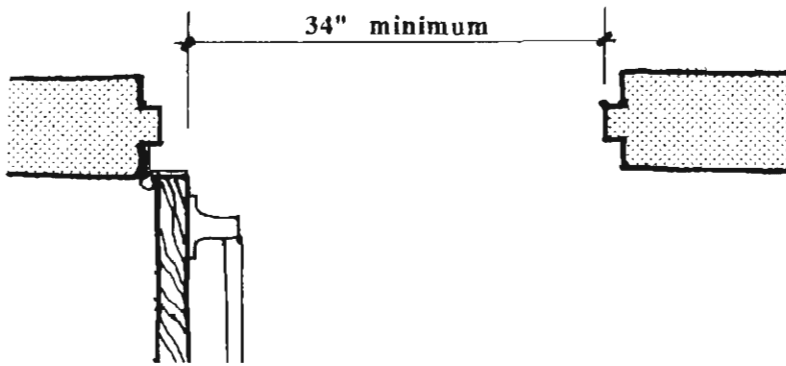
Clear Opening
