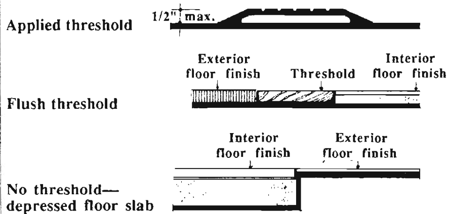
Exterior Thresholds
