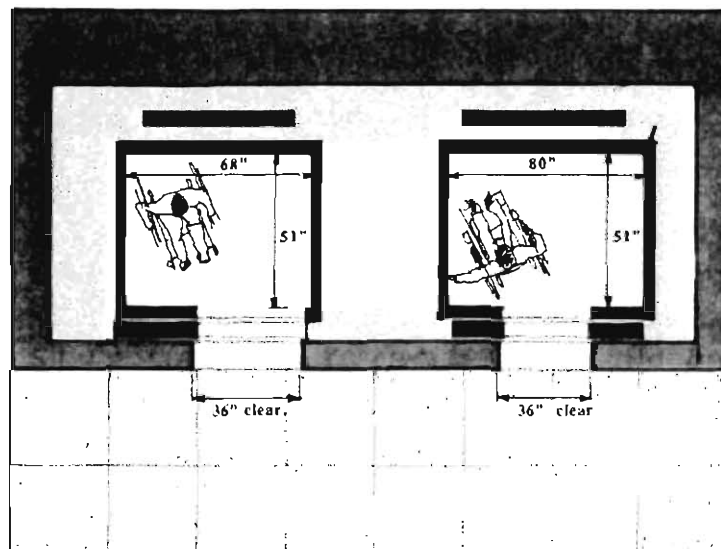
UFAS Elevator Cab Dimensions
