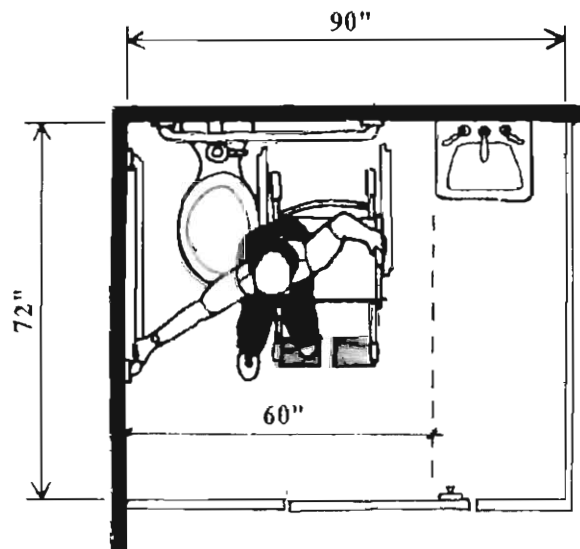
Accessible Stall With Sink
