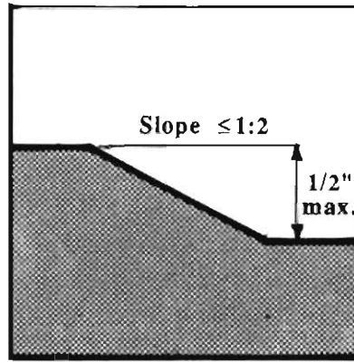
Level Change Beveled With a Slope of 1:2
