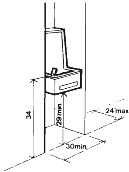
Alcove Installation of Drinking Fountain
