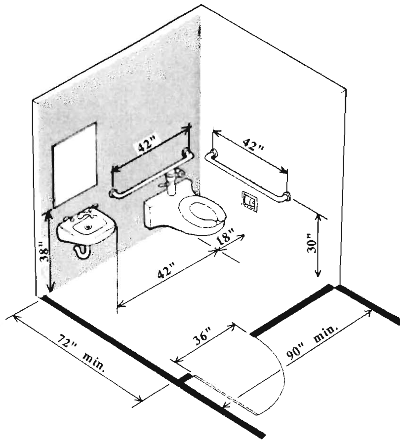
Private Toilet Room
