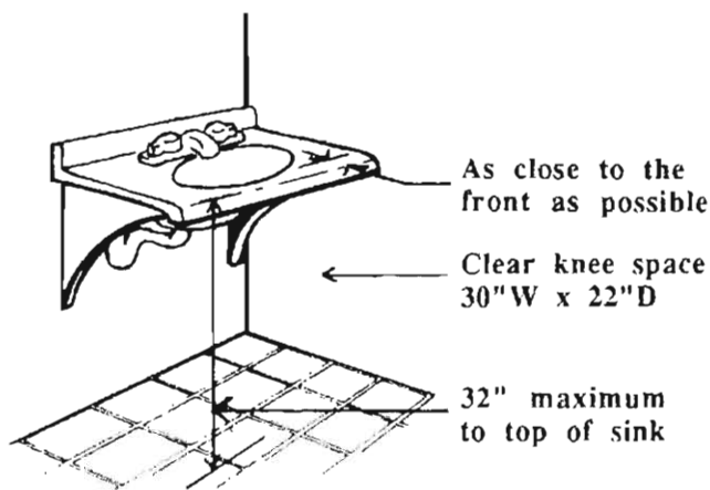
Standard Accessible Sink
