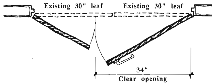
Wide Leaf and Narrow Leaf in an Existing Double Door Frame
