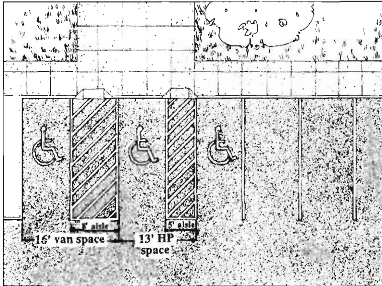
Accessible Parking Space Dimensions
