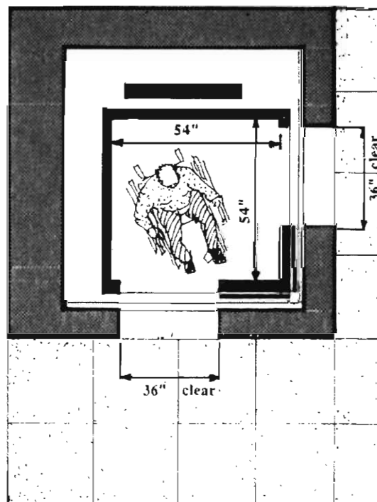
Minimum Dimensions for Two-Door Cab With Doors at Right Angles
