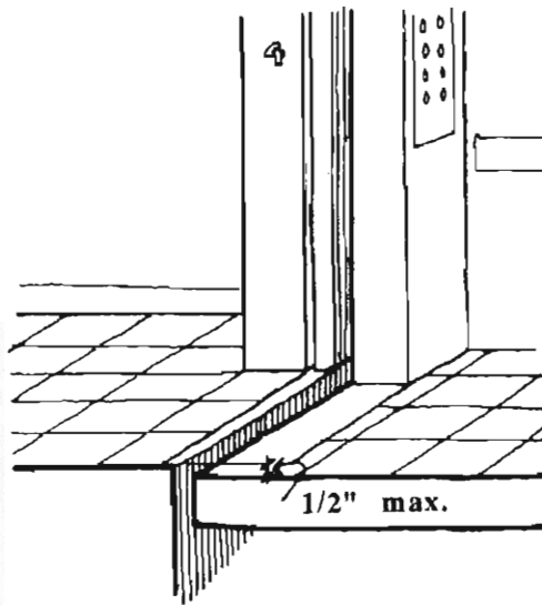
Cab Leveling
