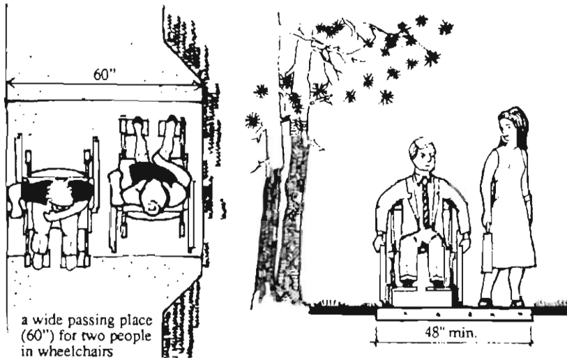
Minimum Pathway Width, With Wider Passing Space
