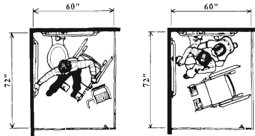
60 Inch Toilet Stalls
